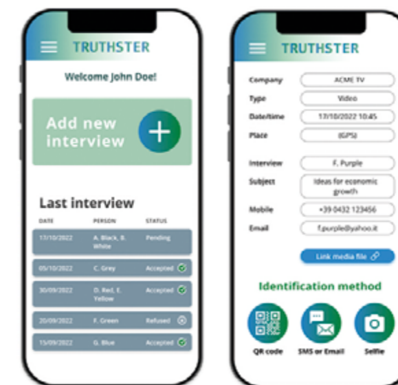
Figure 3: Application interface
