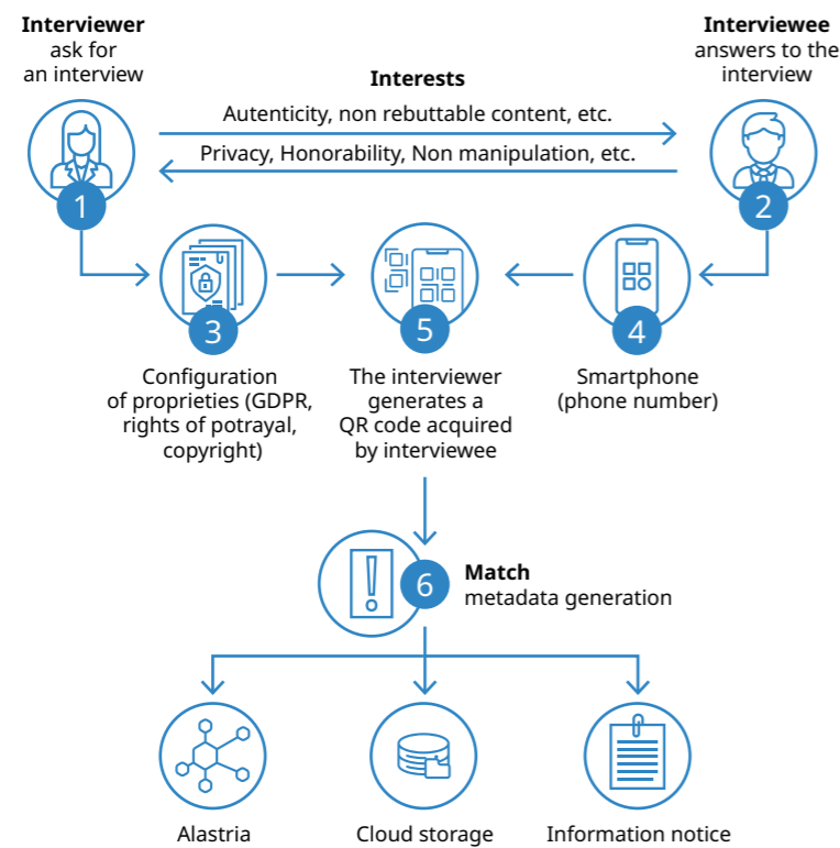
Figure 1: Platform schema
