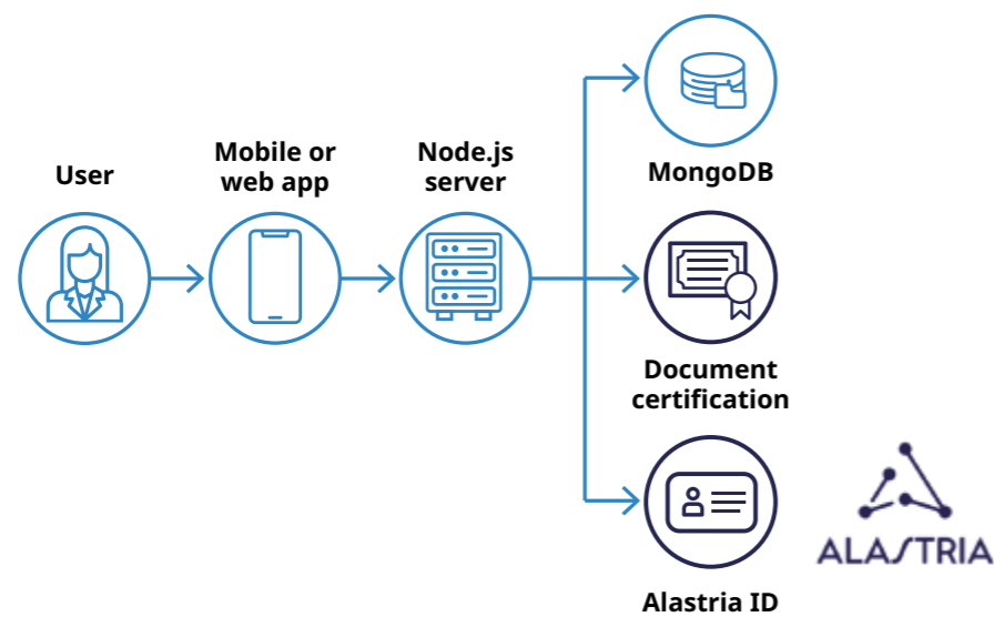
Figure 2: Back-end schema
