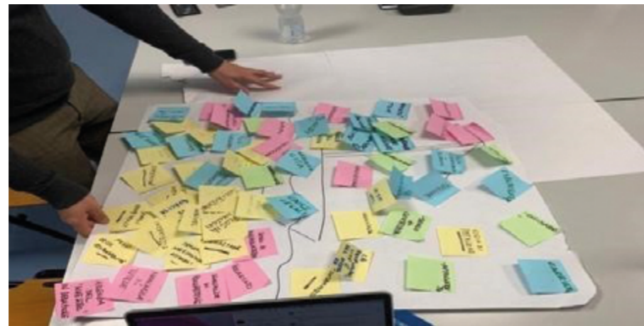
Figure 4: Design thinking
